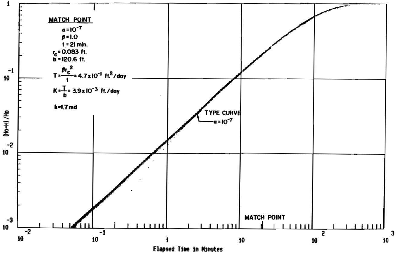
FIGURE 11 EARLY-TIME SLUG TEST PLOT FOR DST-4178/SFL
