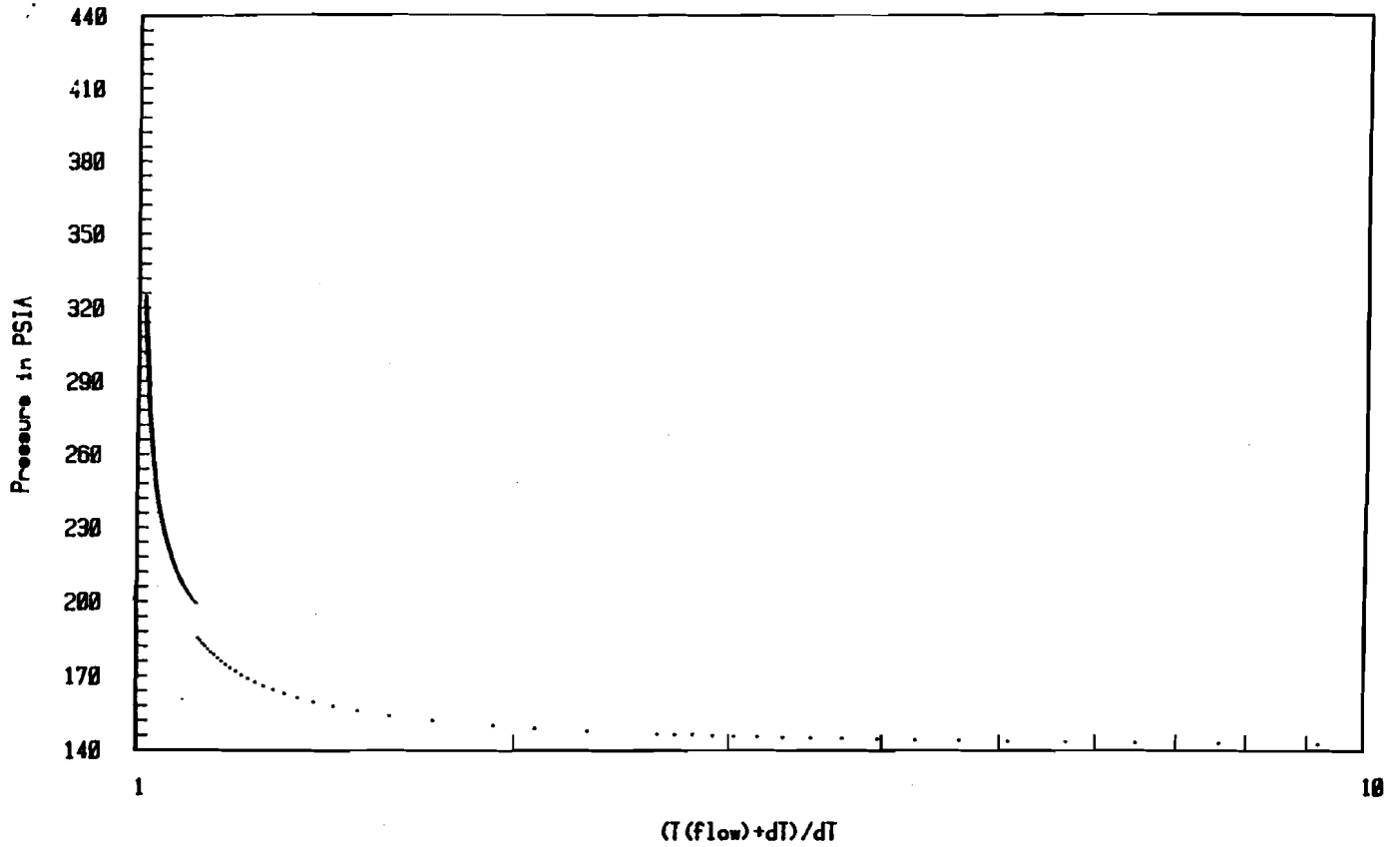
FIGURE 27 HORNER PLOT OF DST-765/SBU
