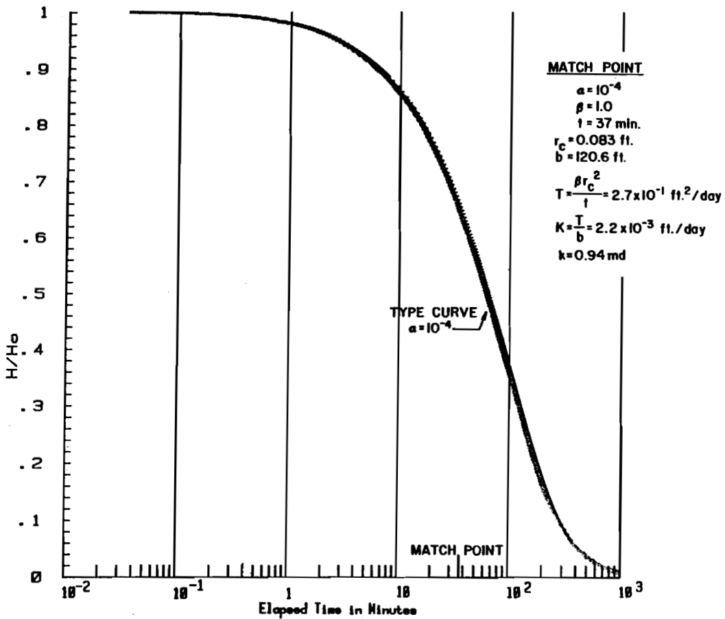
FIGURE 12 SLUG TEST PLOT FOR DST-4178/SLUG
