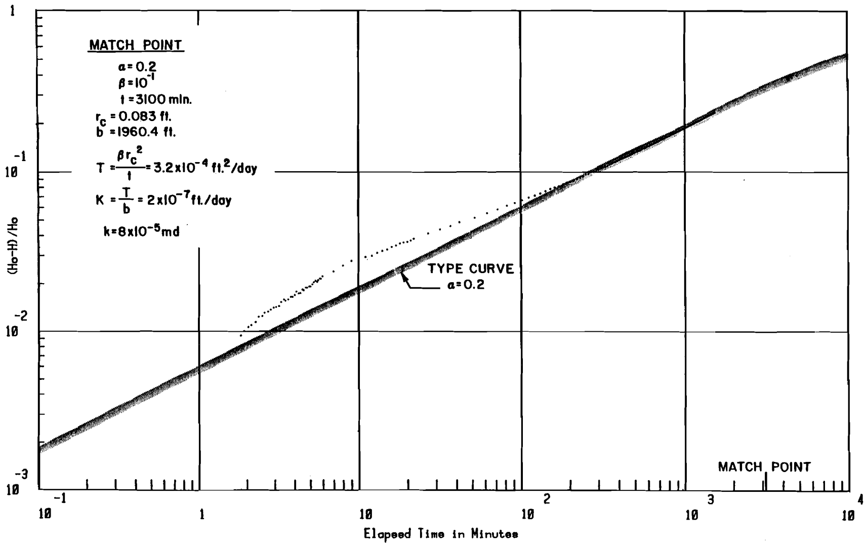
FIGURE 29 EARLY-TIME SLUG TEST PLOT FOR DST-765/SLUG
