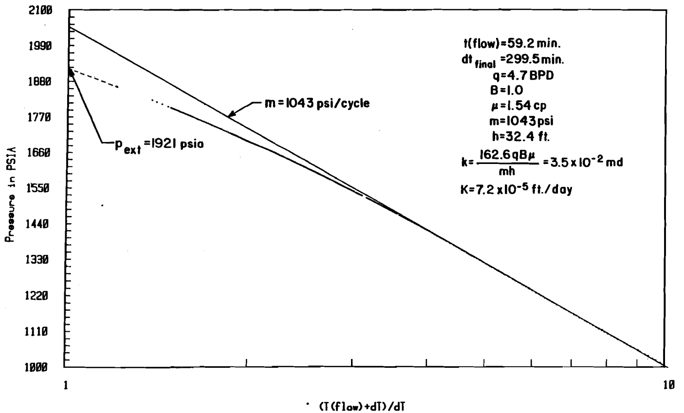
FIGURE 15 HORNER PLOT OF DST-4138/SBU
