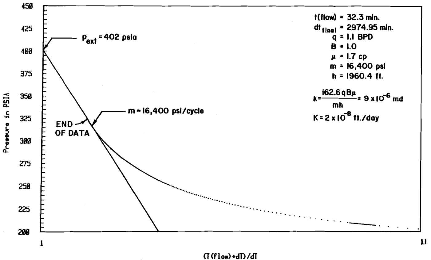
FIGURE 28 EXPANDED-SCALE HORNER PLOT OF DST-765/SBU
