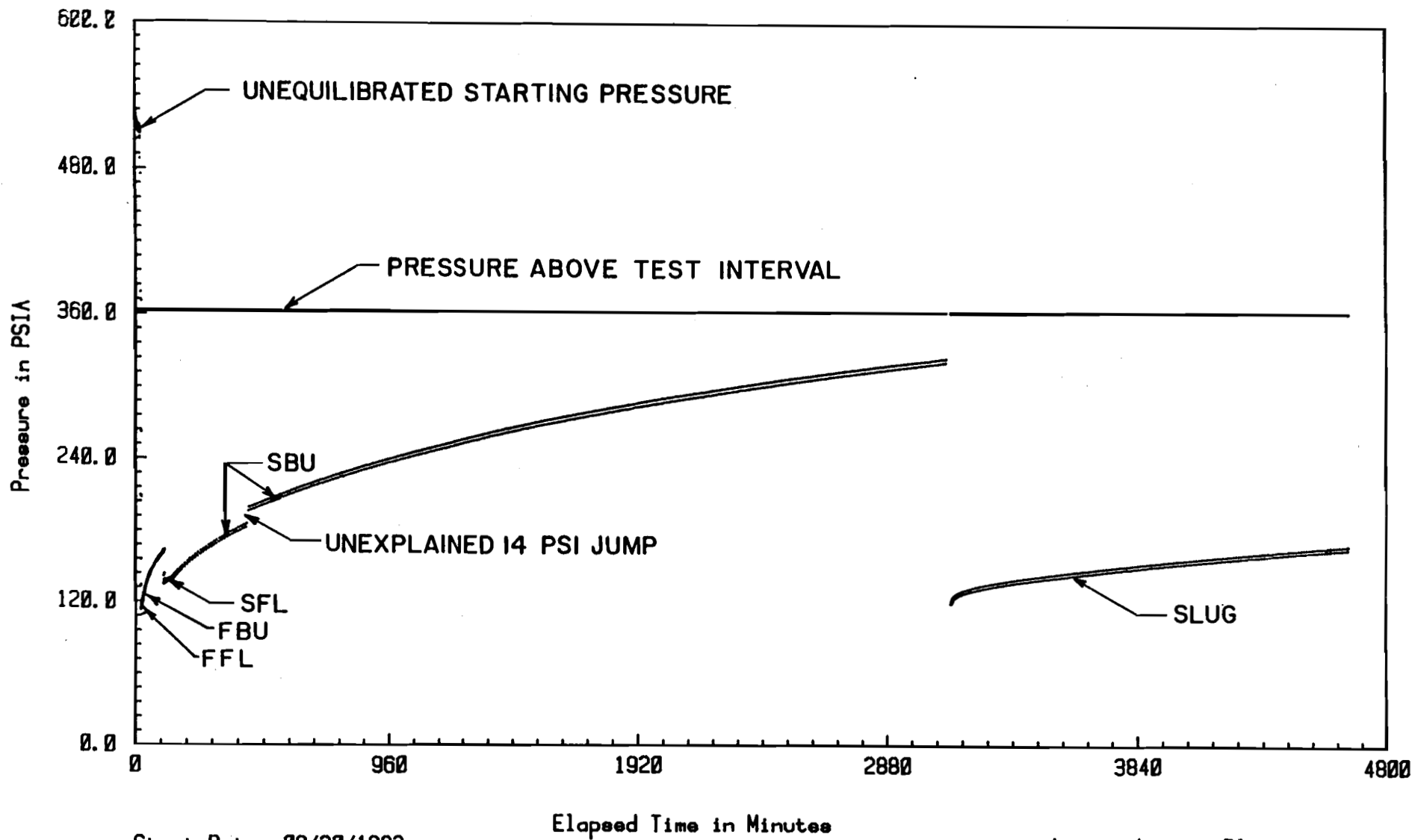
FIGURE 26 REAL-TIME PLOT OF DST-765: SALADO FORMATION
